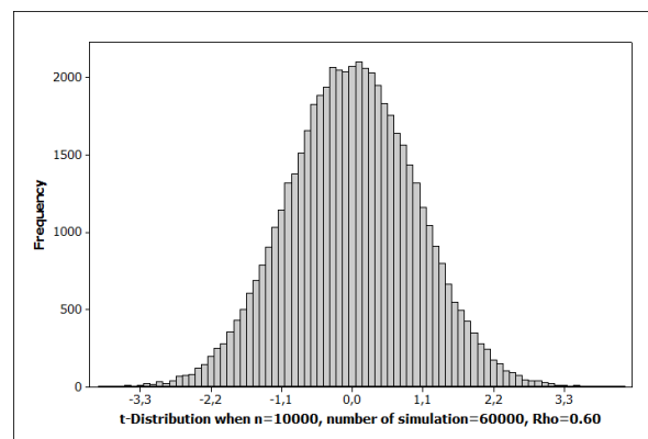
Figure 1: Empirical sampling distributions of Mean/SEmean statistics when n=10,000 , number of simulation is 60,000 and Rho=0.60 (Close to standard normal distribution)
