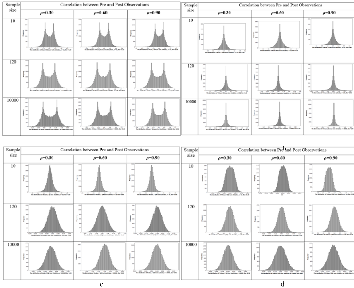
Figure 3: Empirical sampling distribution of (a) Mean/SEmean statistics, (b) TrMean/SEmean statistics, (c) Median/IQR statistics and (d) TrMean/IQR statistics for MSPC
