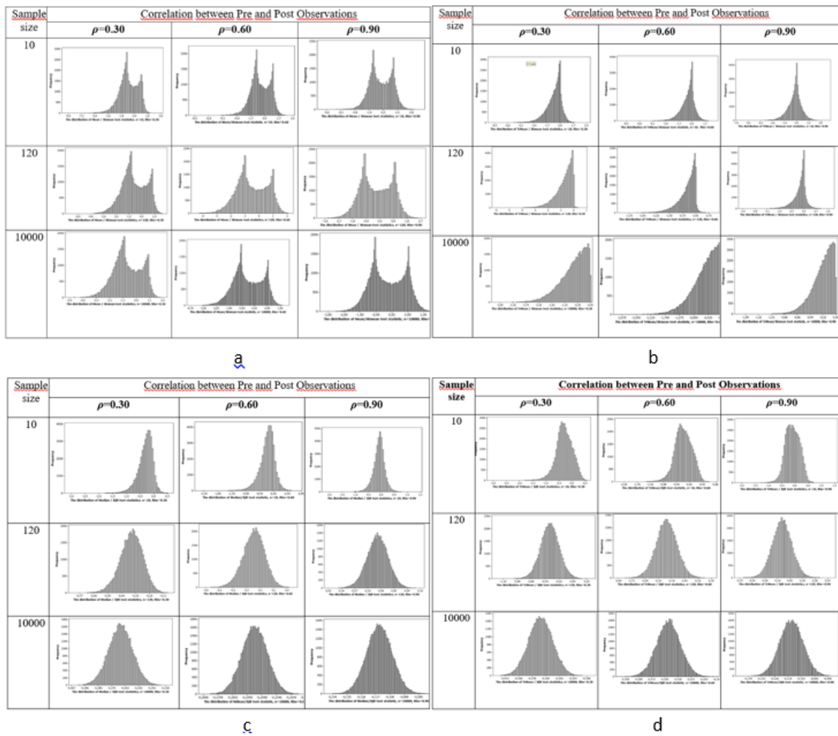
Figure 2: Empirical sampling distributions of a) Mean/SEmean statistics, b) TrMean/SEmean statistics, c) Median/IQR statistics and d) TrMean/IQR statistics for using PC
