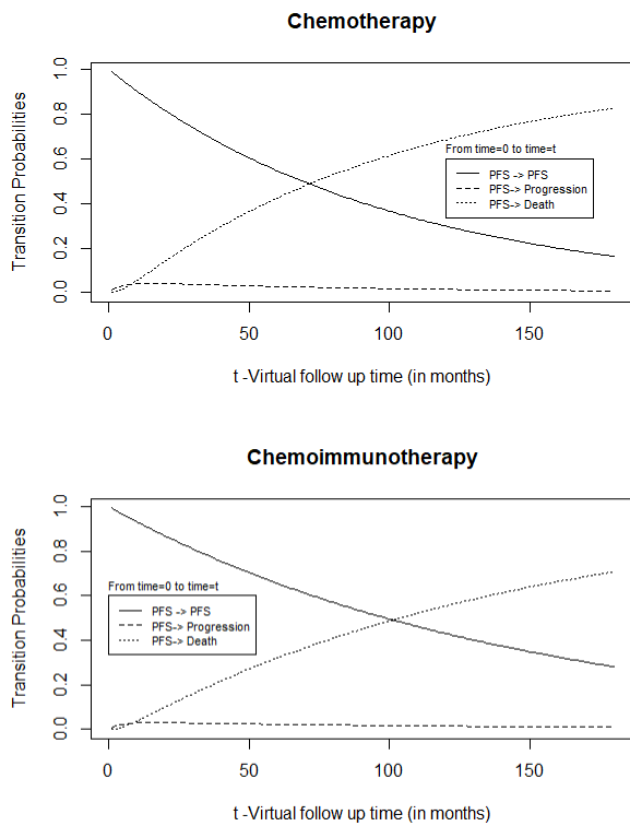
Figure B.2: Transition probabilities plotted against time—Multinomial-Dirichlet Bayesian model
