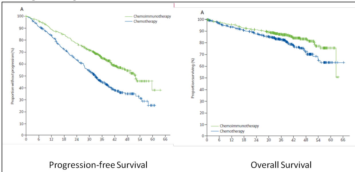
Figure 1: Kaplan-Meier curves used for data reconstruction
