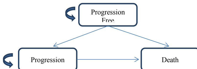
Figure 3: Transition map between three states of the multi-state model
