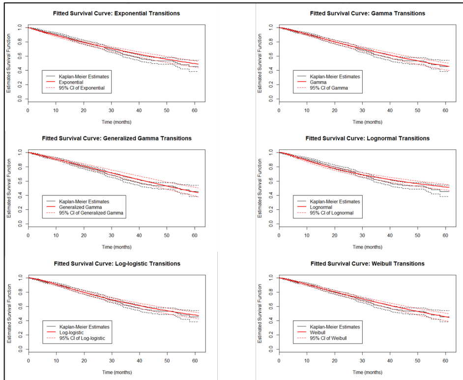
Figure A.1: Estimated survival functions of fitted models—Chemotherapy group
