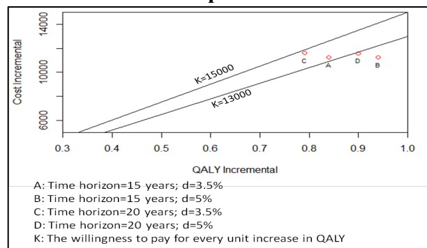
Figure 5: Cost-effectiveness plane from the first method
