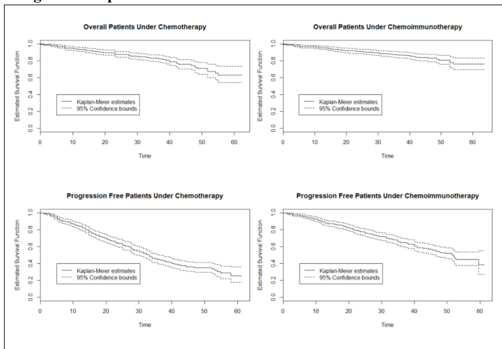
Figure 2: Kaplan-Meier curves from reconstructed data
