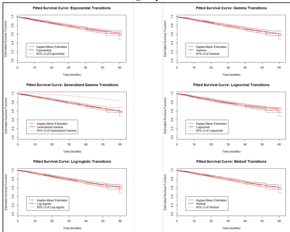
Figure A.2: Estimated survival functions of fitted models—Chemoimmunotherapy group
