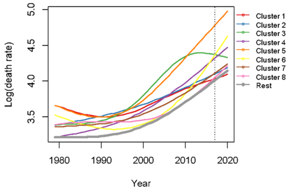
Figure 9: Trends of SAD AAR from 1979 to 2020 between 8 spatial metaclusters (as curves of different colors) are compared with the “Rest” of the Appalachian counties (bold grey curve). The predicted death rates for the time-period beyond 2017 are shown to the right of the dotted line.
